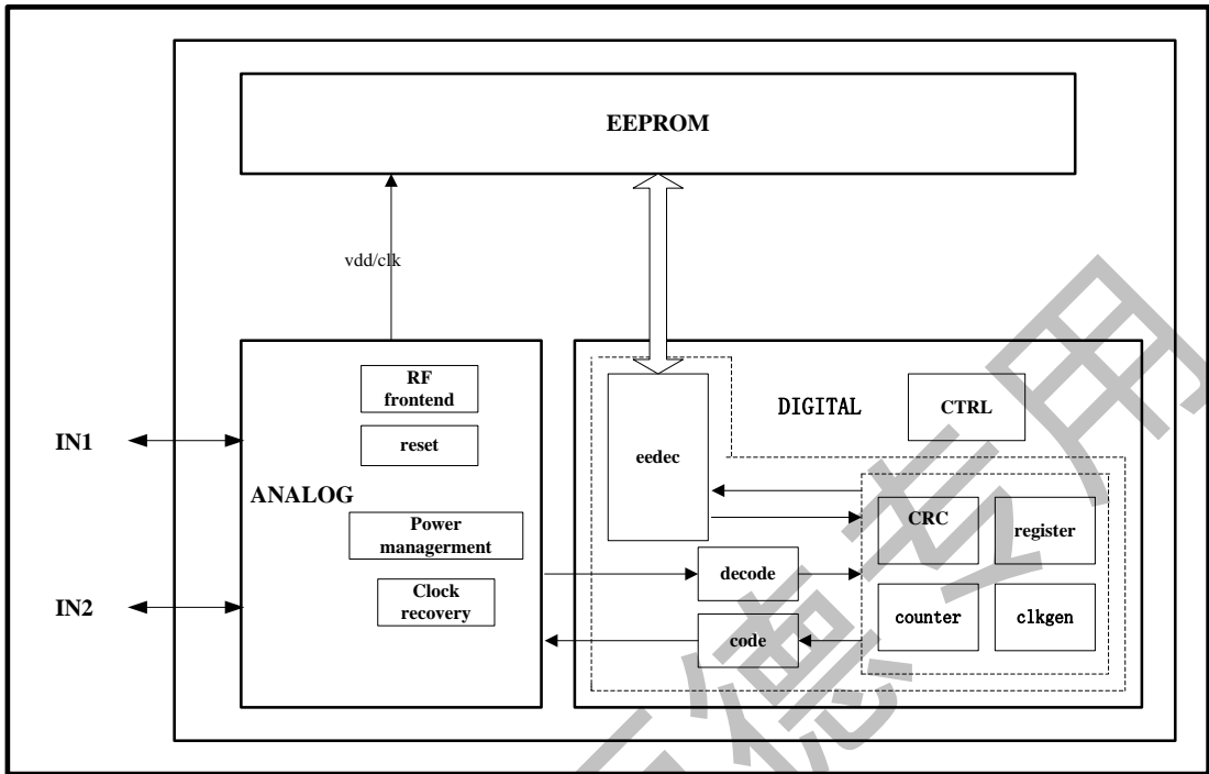
Figure 1-1 RF08S Block diagram
